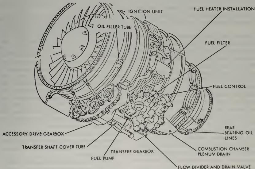
FIGURE 1-35. Accessory arrangement on an axial-flow engine.
